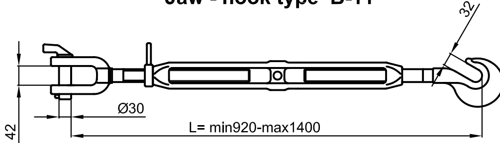
Jaw - hook type B-11
