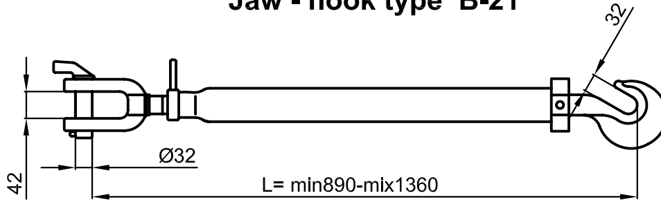
Jaw - hook type B-21
